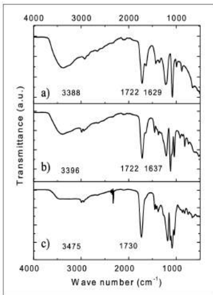
Fig. 1. IR-spectra of a) glycolic acid, b) L-lactic acid, c) 70:30%wt.L-LA:%wt.GA. PLLGA copolymer and d) reaction scheme of PLLGA
